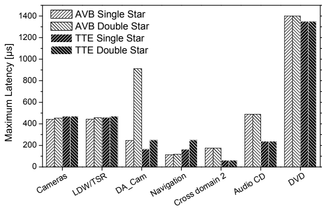
Fig. 3. Comparison of maximum latency of all flows in Case A
