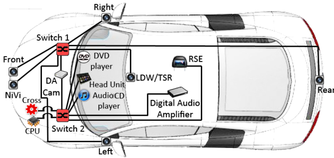
Fig. 1. Single Star Topology
