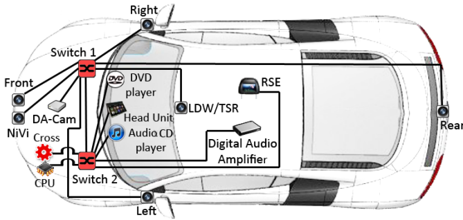
Fig. 2. Double Star Topology
